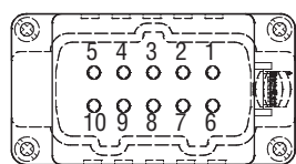
10P female View on terminals
