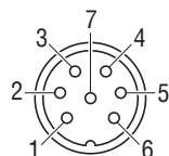
Front side molded 7P Male connector
