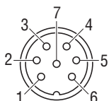
Solder side 7P Female connector
