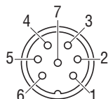
Solder side 7P Male connector
