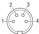
Camera 1 + 2 Front side 4p Molded Female connectors
