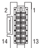
Crimp side Female connector Monitor side 16p connector housing
